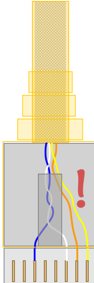
Figure 41: badly assembled RJ45 connector
