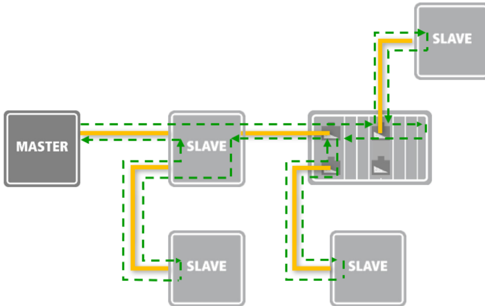
Figure 7: EtherCAT frame routing
