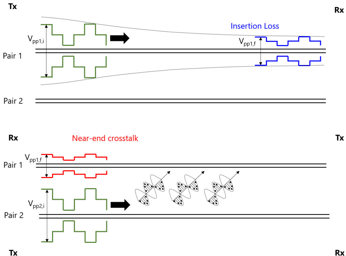
Figure 11: physical meaning of IL and NEXT parameters
