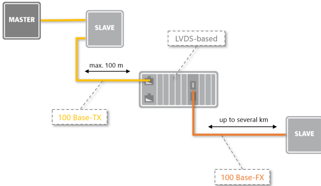
Figure 2: EtherCAT physical media
