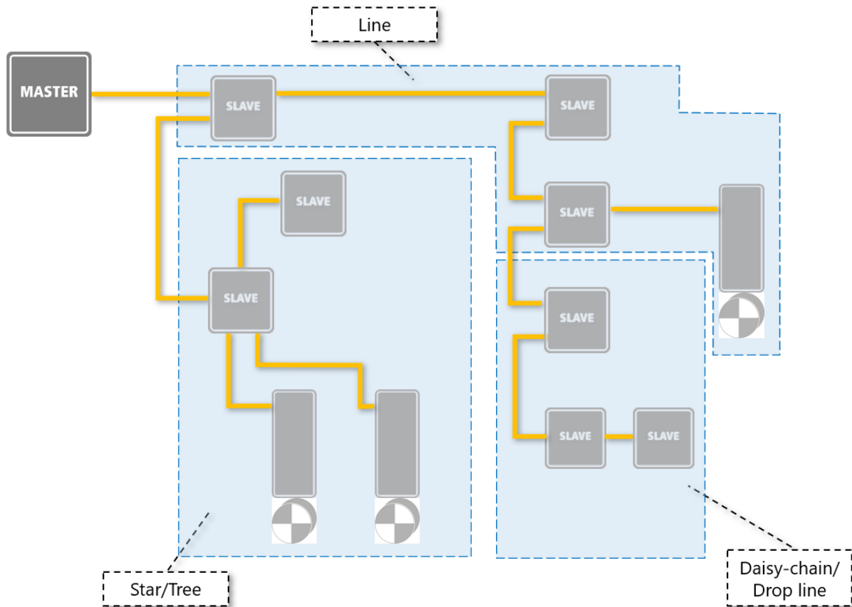
Figure 3: EtherCAT topologies
